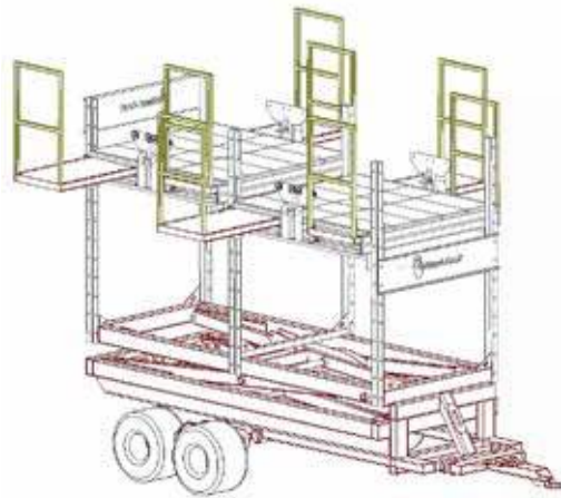
BOG Mounted Platform
